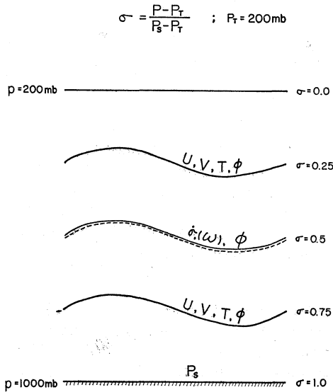
Fig. 1. Schematic representation of vertical structure of the 2-level primitive equation model.
