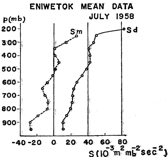
Fig. 7. Vertical profile of the mean monthly value of static stability factor for Eniwetok Island ( 12.0^\circ \text{ N} , 162.0^\circ \text{ E} ) for the month of July, 1958 (by Yanai, 1961).
