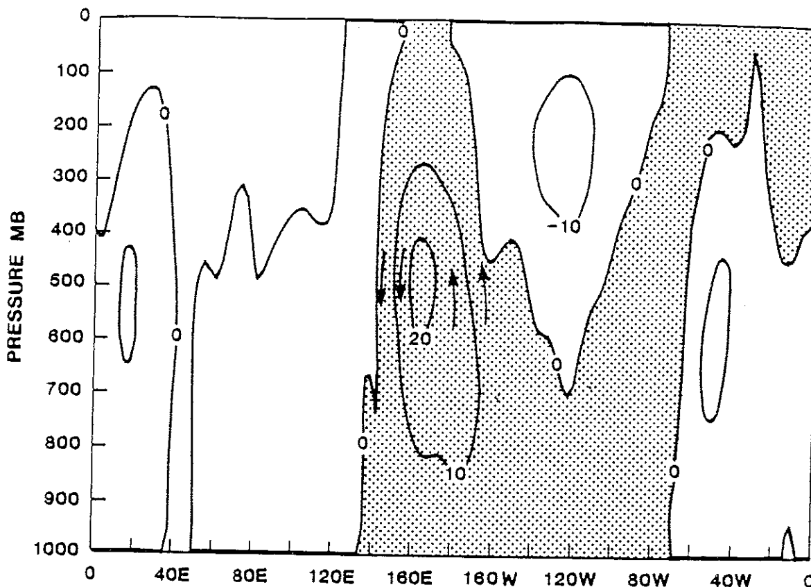
Figure 5d. Difference (anomaly-control) of Walker cell (in units of 10^9 kg/sec) averaged between 6^\circ\text{N} - 6^\circ\text{S} and averaged for days 6-25
