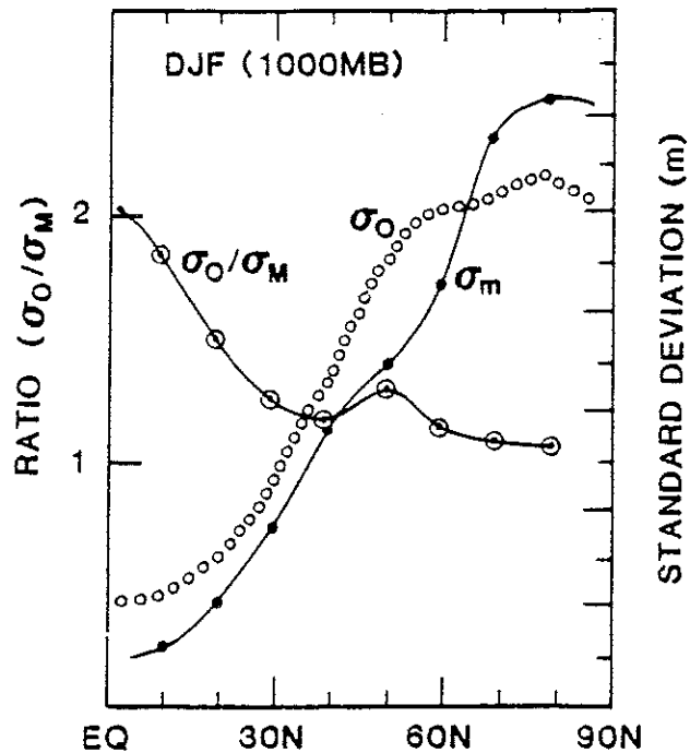
Figure 10a. Zonal means of standard deviation of monthly mean 1000 mb geopotential height (m) for the Dec.-Jan.-Feb. season. Observed distributions are from Oort and Jenne. The ratio of observed and model standard deviation is on the left hand side. (from Manabe and Hahn, 1981)
