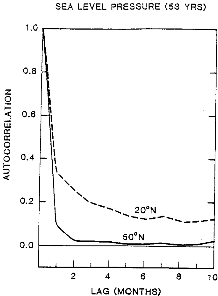
Figure 11b. Zonally averaged autocorrelation at 20°N and 50°N for monthly mean sea level pressure for the period 1925-77
