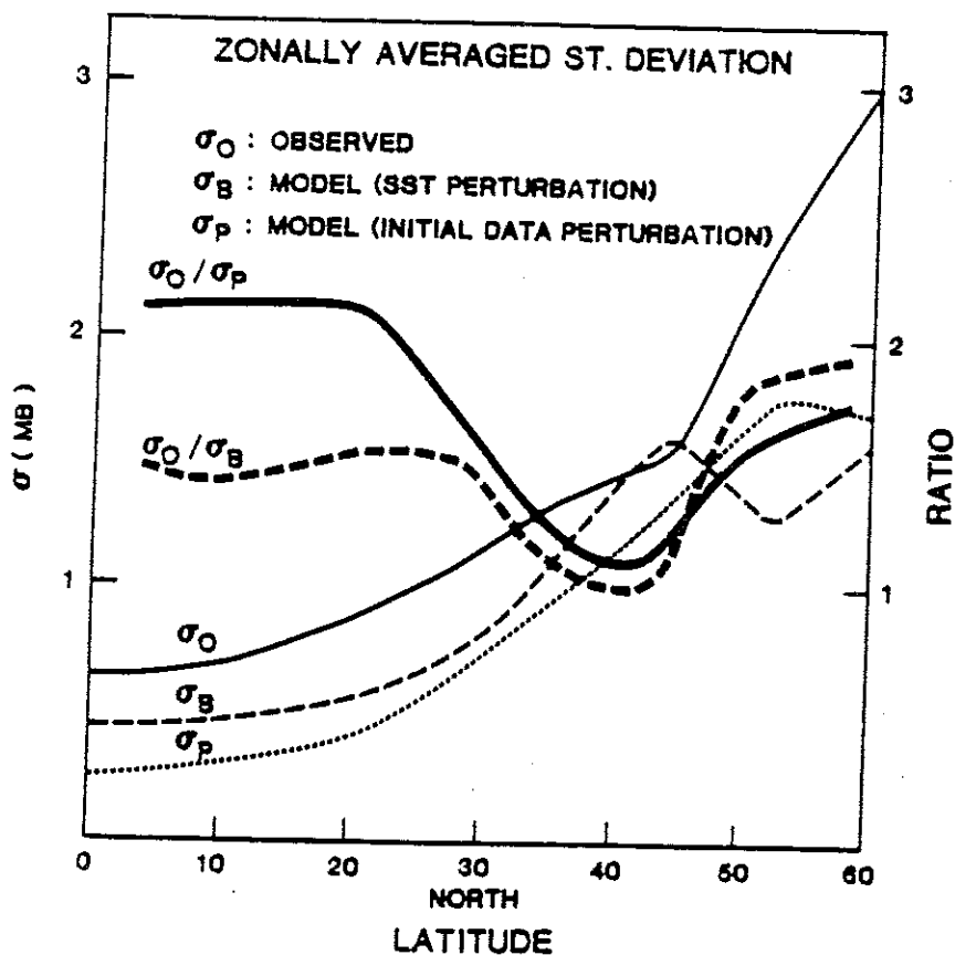
Figure 9. Zonally averaged standard deviation among monthly mean (July) sea level pressure (mb) for 10 years of observations ( \sigma_O , thin solid line); four model runs with variable boundary conditions ( \sigma_B , thin dashed line); and four model runs with identical boundary conditions ( \sigma_P , thin dotted line). Thick solid line and thick dashed line show the ratio \sigma_O/\sigma_P and \sigma_O/\sigma_B respectively
