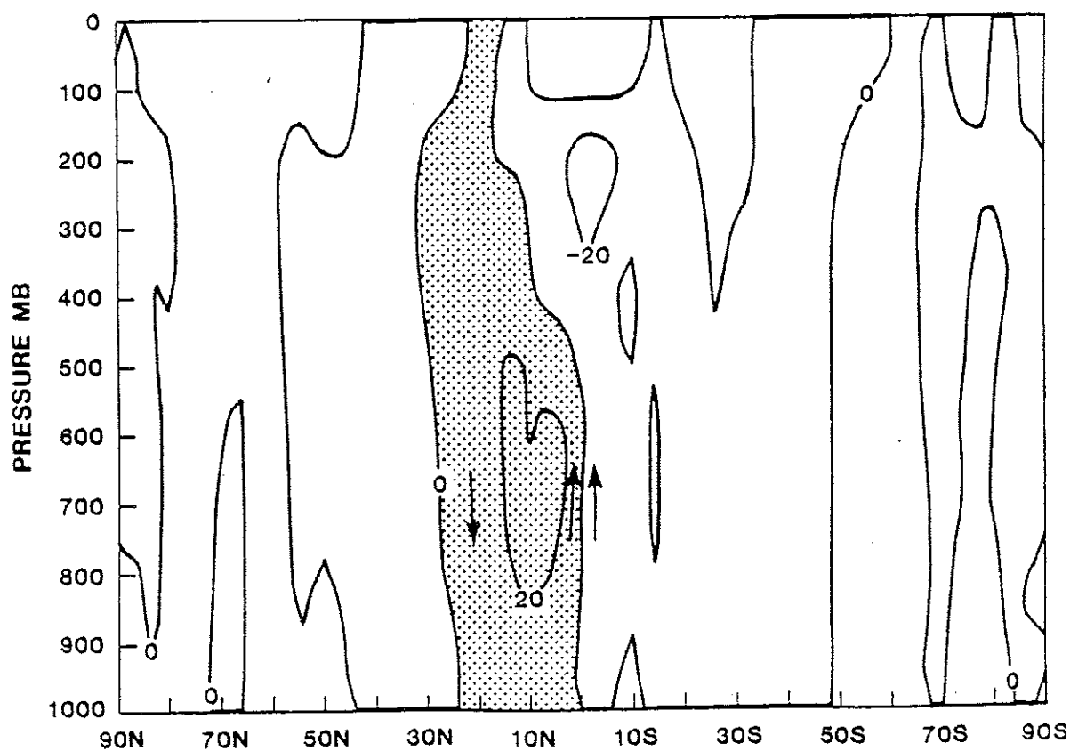
Figure 5c. Difference (anomaly-control) of Hadley cell (in units of 10^9 kg/sec) averaged for days 6-25.
