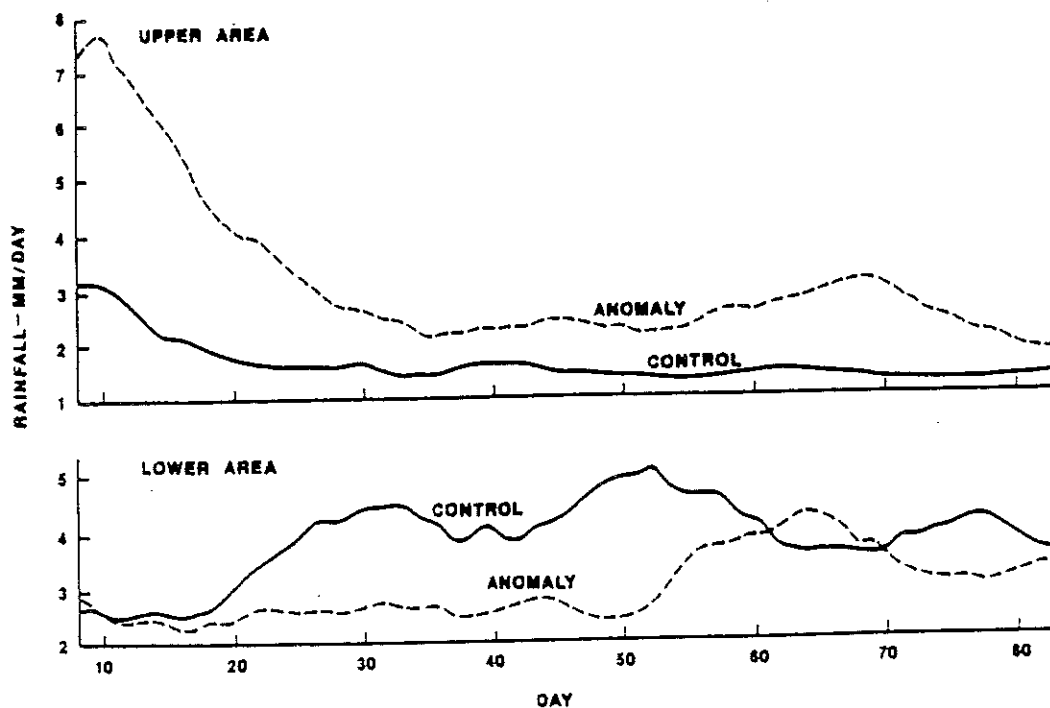
Figure 4b. 15 day running mean of daily rainfall (mm/day) for upper area (A) and lower area (B). (From Moura and Shukla, 1981)
