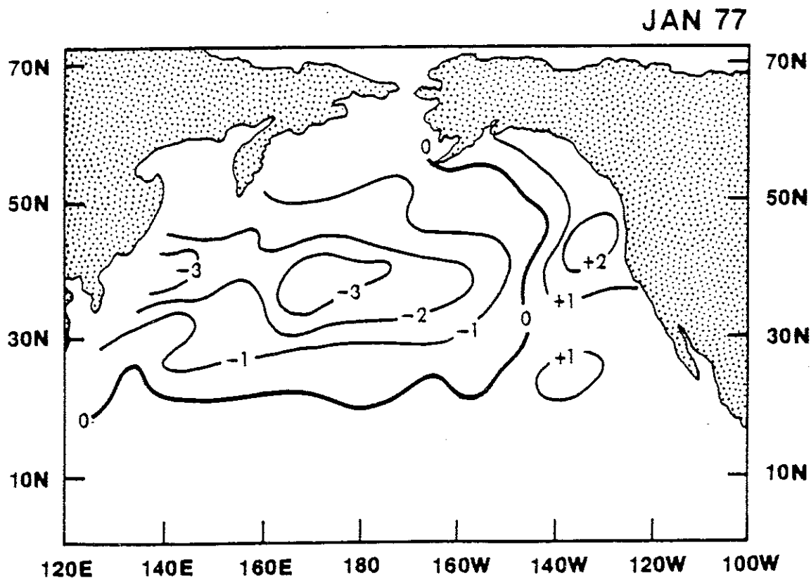
Figure 6a. Sea surface temperature anomaly ( ^{\circ}\text{C} ) over the north Pacific used for the GCM experiment. This anomaly pattern will be identical to the observed SST anomaly during January 1977 if the units are changed from ( ^{\circ}\text{C} ) to ( ^{\circ}\text{F} )
