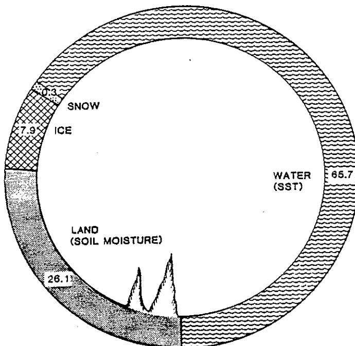
Figure 1a. Schematic representation of the atmosphere's lower boundary. Numbers denote the percentage of earth surface area covered by different boundary forcings during January
