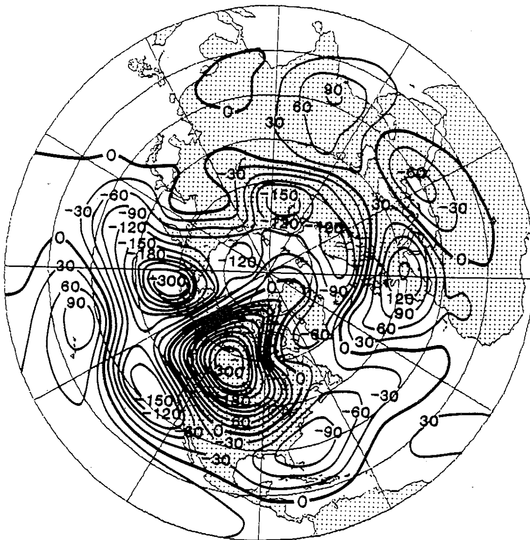
Figure 5b. Difference (anomaly-control) of 300 mb geopotential height field averaged for days 11-25
