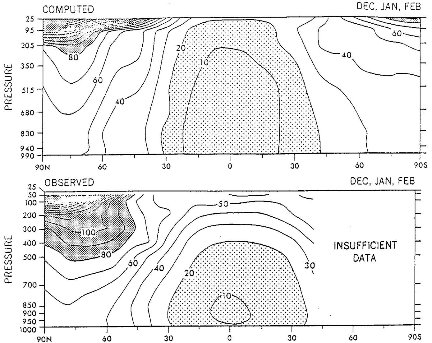
Figure 10b. Zonal mean of the standard deviation of monthly mean geopotential height (m) for the Dec.-Jan.-Feb. season. Top: simulated; Bottom: observed (from Manabe and Hahn, 1981)
