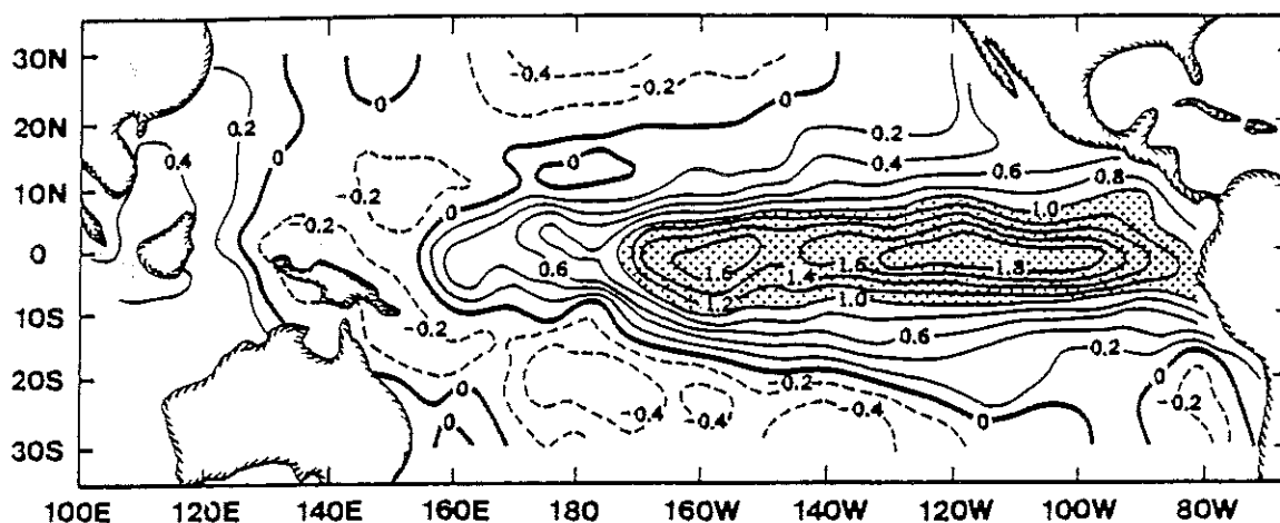
Figure 5a. Sea surface temperature anomaly ( ^{\circ}\text{C} ) used for the GCM experiment
