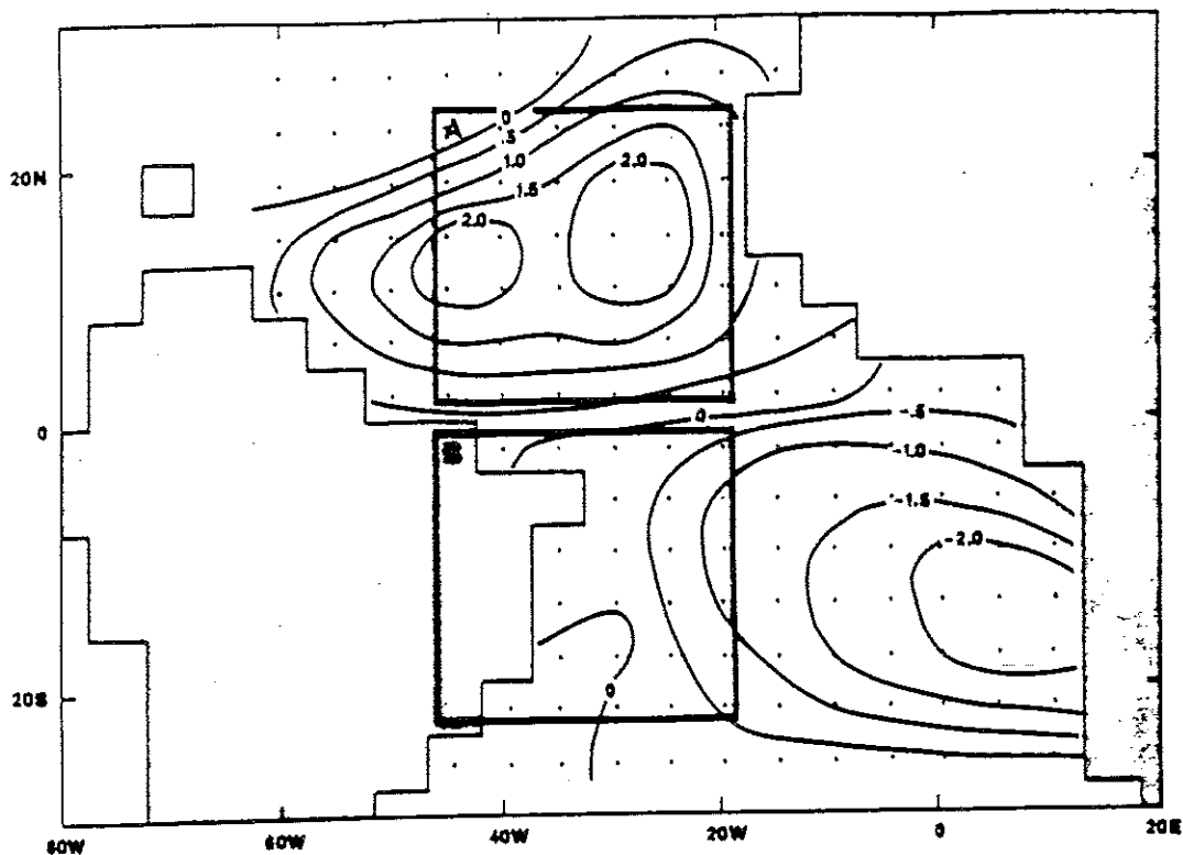
Figure 4a. Sea surface temperature anomaly ( ^{\circ}\text{C} ) over the tropical Atlantic used for the GCM experiment
