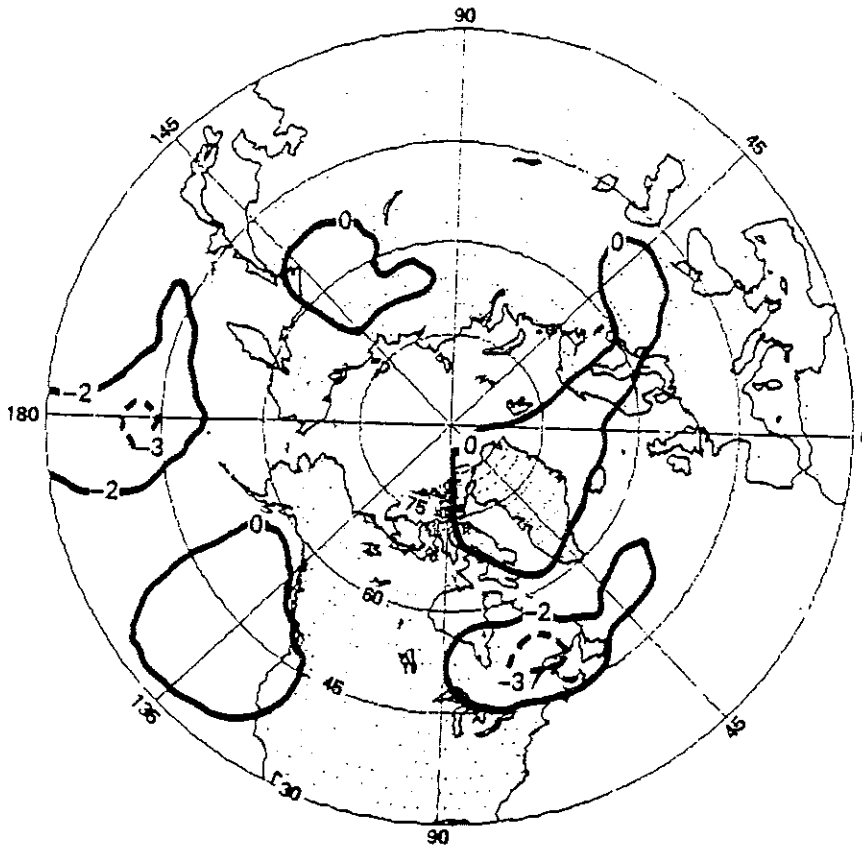
Figure 6c. Ratio of the temperature difference at 700 mb (shown in Figure 6b) to the standard deviation among 15-45 day averages of six control runs
