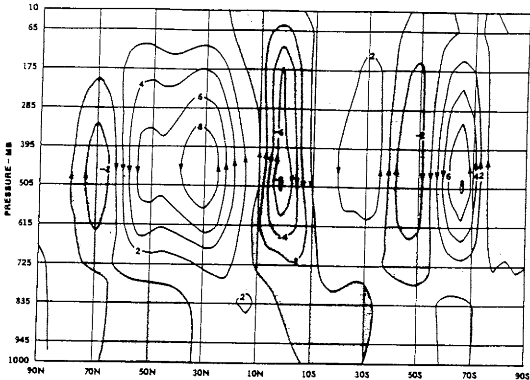
Figure 4c. Difference of 60 day mean meridional circulation ( 10^{13} gm/sec) averaged between the longitudes 50^{\circ} W and 5^{\circ} W. (From Moura and Shukla, 1981)
