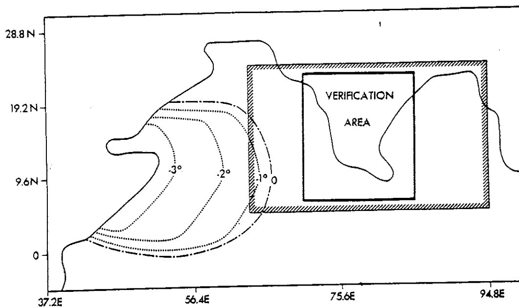
Figure 2a. Sea surface temperature anomaly ( ^{\circ}\text{C} ) over the Arabian Sea used for the GCM experiment and the area of verification
