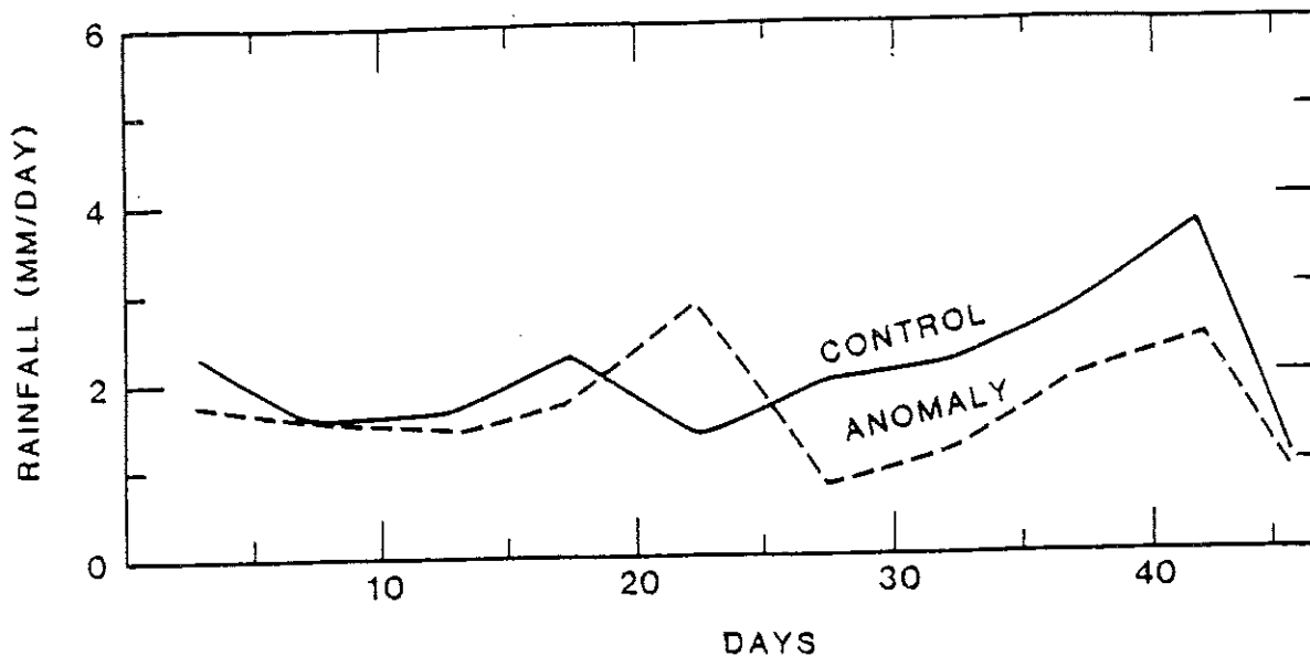
Figure 7f. Five day average rainfall over northeast Brazil, for control and anomaly run
