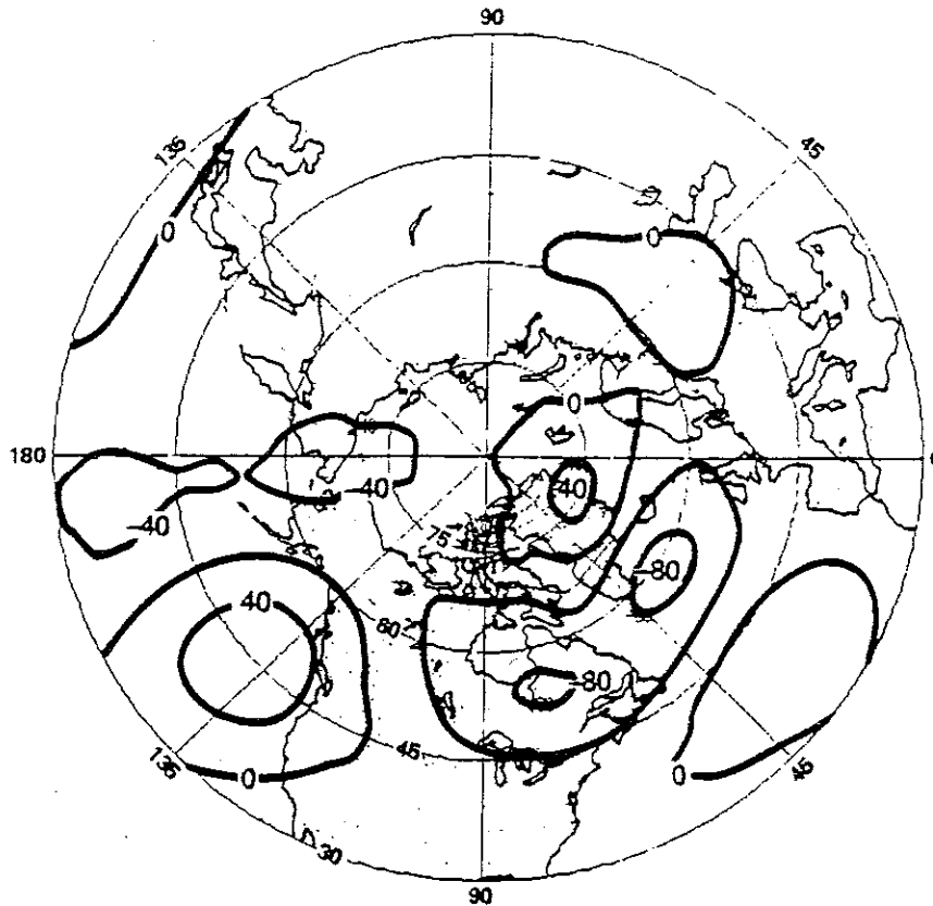
Figure 6d. Geopotential height difference (meters) at 500 mb between the average of two anomaly runs and the average of the six control runs averaged for days 15-45
