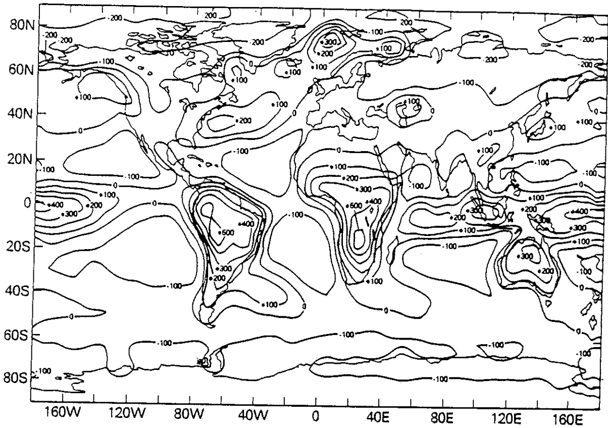
Figure 7a. Vertically integrated net diabatic heating ( \text{cal cm}^{-2} \text{ day}^{-1} ) of the atmosphere during winter, as simulated by the GLAS climate model
