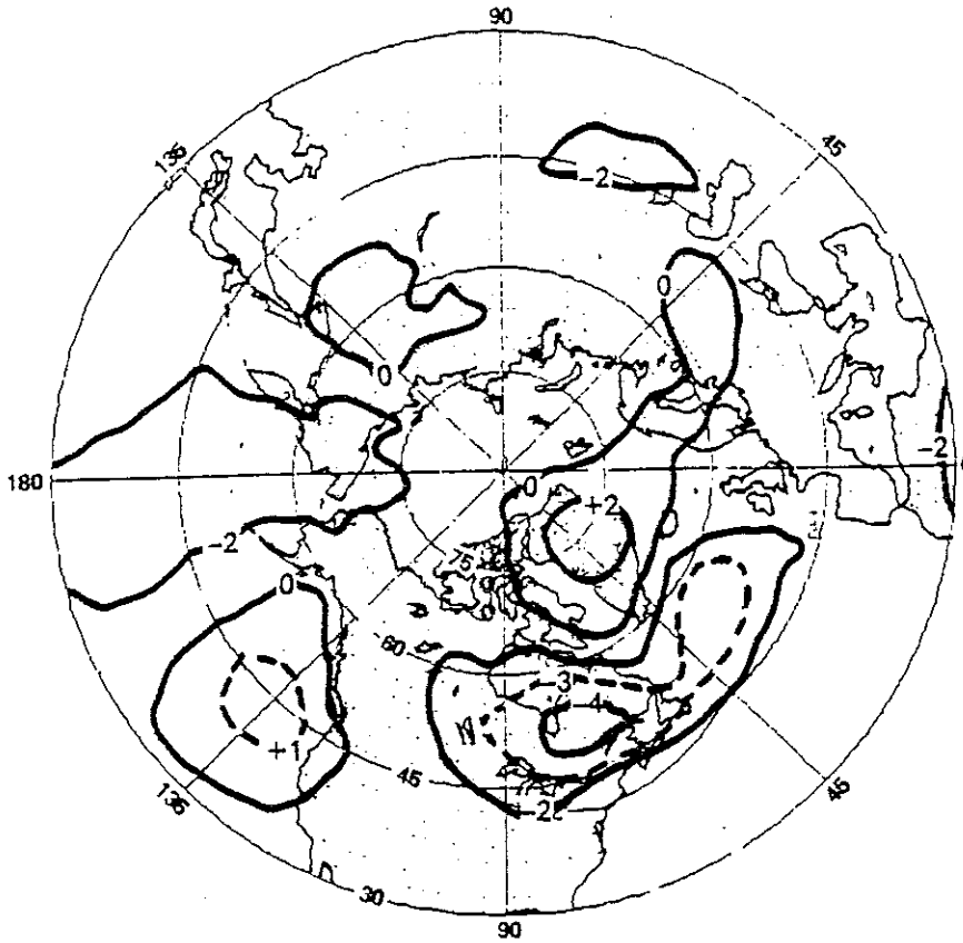
Figure 6b. Temperature difference ( ^{\circ}\text{C} ) at 700 mb between the average of the two anomaly runs and the average of the six control runs, averaged for days 15-45
