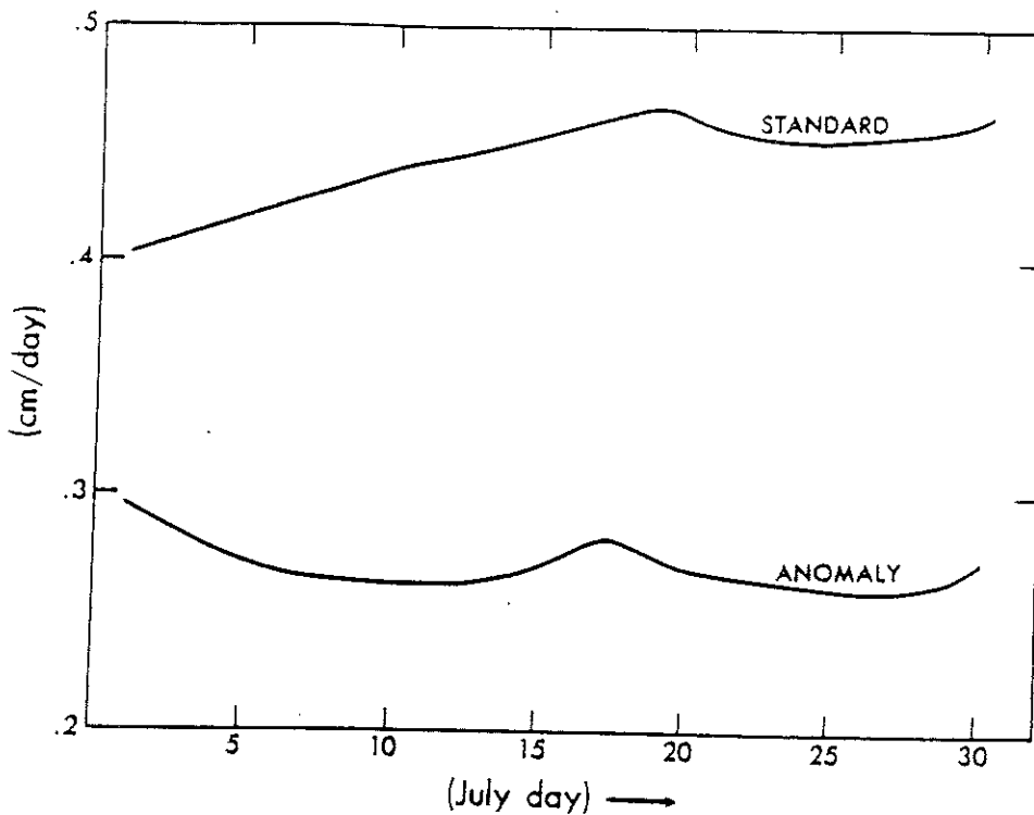
Figure 2b. 15 day running mean of the rate of precipitation ( \text{cm day}^{-1} ) averaged over the verification area for the standard and anomaly runs
