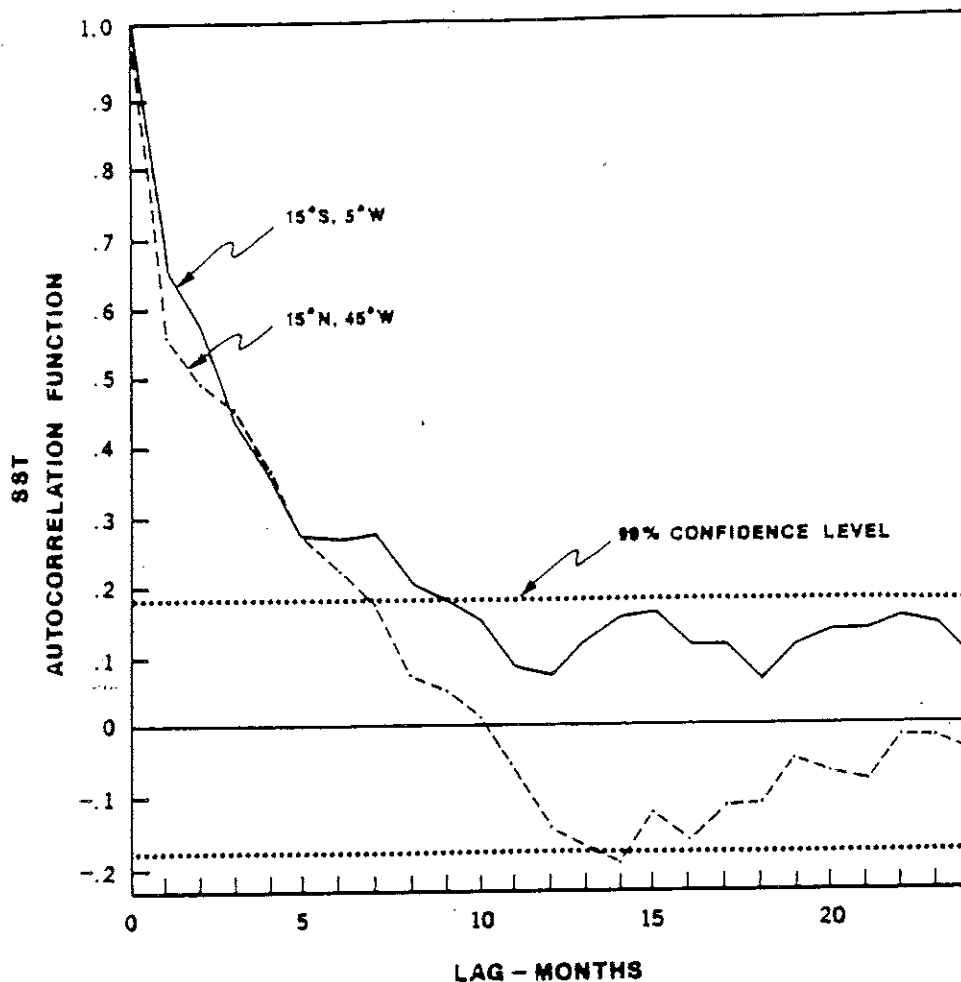
Figure 4d. Lag correlation function for monthly mean SST anomaly at 15^{\circ}\text{S} , 5^{\circ}\text{W} and 15^{\circ}\text{N} , 45^{\circ}\text{W} . (From Moura and Shukla, 1981)
