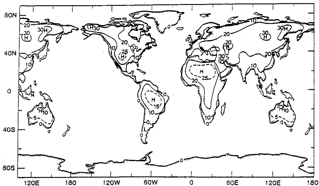
Figure 7d. Ground temperature difference ( ^{\circ}\text{C} ) between two model simulations (dry soil-wet soil) for the month of July
