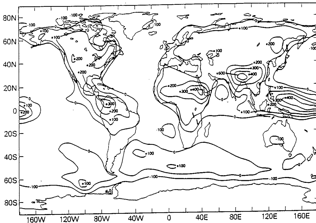
Figure 7b. Vertically integrated net diabatic heating ( \text{cal cm}^{-2} \text{ day}^{-1} ) of the atmosphere during summer, as simulated by the GLAS climate model
