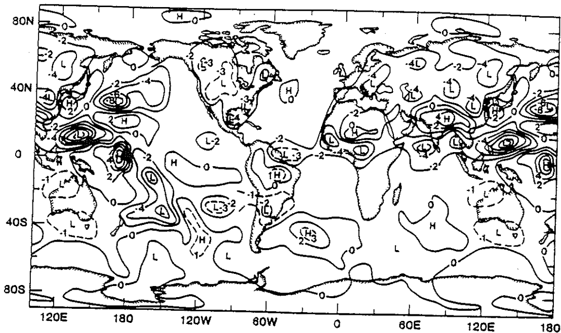
Figure 7c. Rainfall difference (mm/day) between two model simulations (dry soil-wet soil) for the month of July
