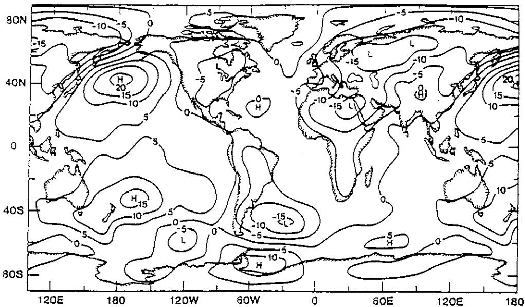
Figure 7e. Surface pressure difference (mb) between two model simulations (dry soil-wet soil) for the month of July
