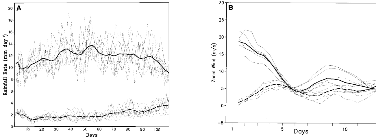
Fig. 2. (A) Daily values of area averaged ( 10^{\circ}\text{S} to 10^{\circ}\text{N} , 120^{\circ}\text{W} to 160^{\circ}\text{W} ) rainfall ( \text{mm day}^{-1} ) using observed SST for 1982–1983 (thick solid curve) and 1988–1989 (thick dashed curve). Thick lines represent average of nine members (thin lines) of each ensemble. (B) Daily values of area averaged ( 10^{\circ}\text{S} to 10^{\circ}\text{N} , 120^{\circ}\text{W} to 160^{\circ}\text{W} ) zonal wind
