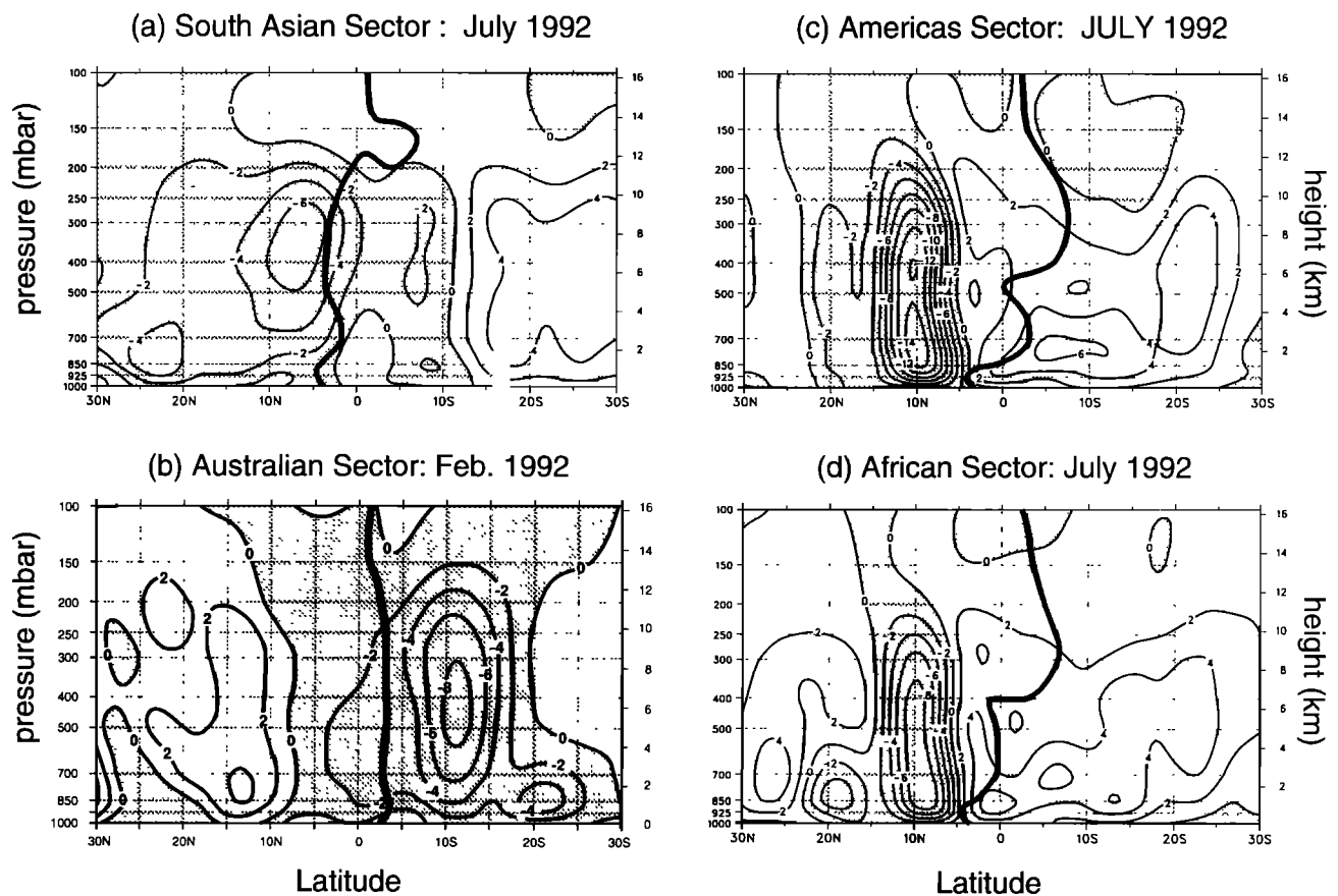
Figure 7. Mean vertical velocity sections through the major monsoonal regions of the globe. (a) the south Asian sector (60° to 85°E) during July, 1992, (b) the Australian sector (120° to 140°E) during February, 1992, (c) the Americas sector (110° to 130°W) during July 1992, and (d) the African sector (30° to 50°W) during July 1992. Units 10^{-6} mbar s^{-1} . The shaded area shows upward motion. The thick line is the zero absolute vorticity contour. Data is from European Center for Medium-Range Weather Forecasts (ECMWF) initialized analyses. Based on the calculations of Tomas and Webster [1997].
