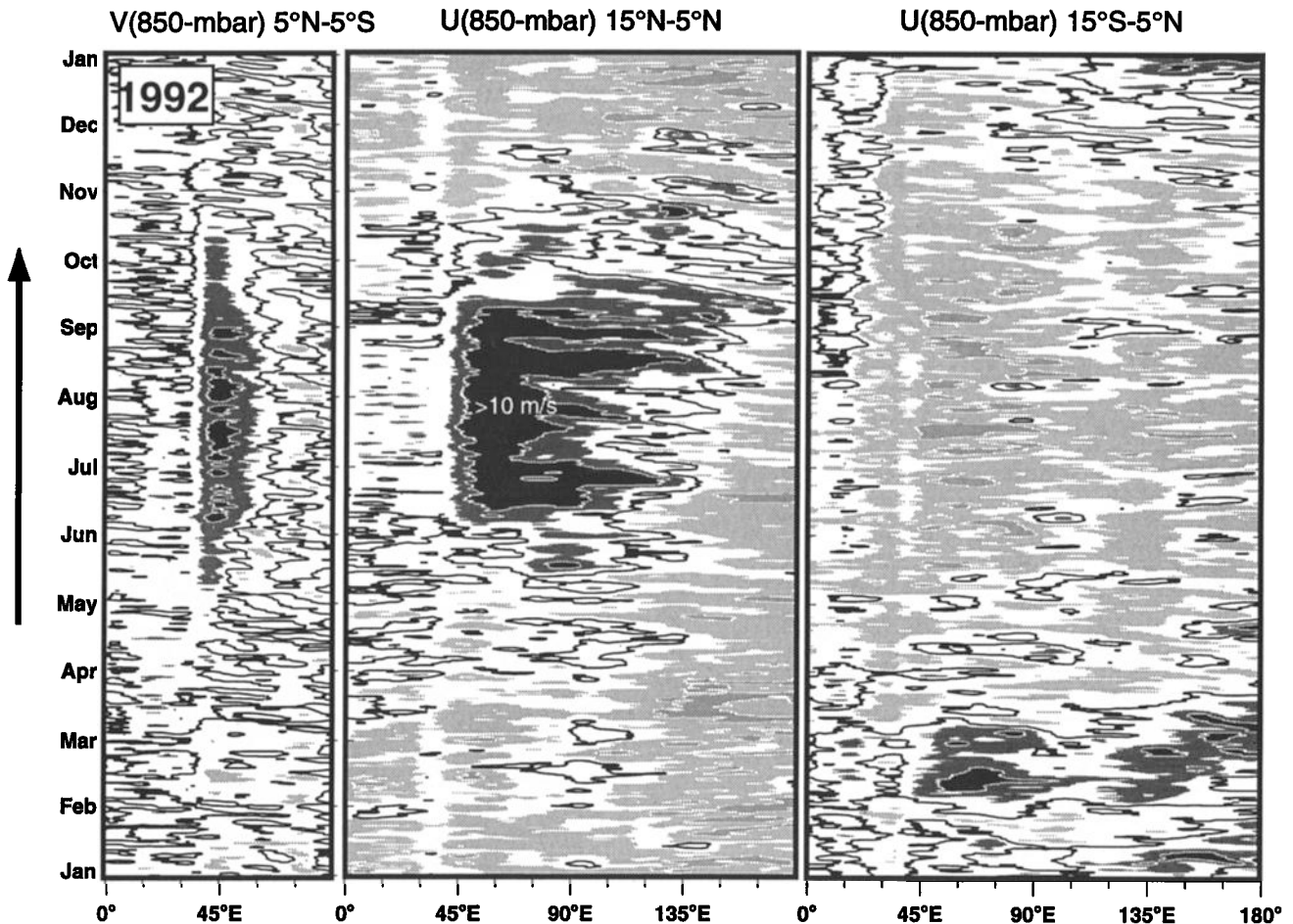
Figure 13b. Space and time distributions of the intraseasonal variability of the monsoon for the year 1992. (left) Longitude-time sections of the 850-mbar meridional velocity component ( V ) along 0\text{--}90^\circ\text{E} averaged between 5^\circ\text{N} and 5^\circ\text{S} . Dark contour denotes zero speed. (middle) 850 mb zonal velocity component ( U ) along 0\text{--}180^\circ averaged between 5^\circ and 10^\circ\text{N} . Dark contour denotes zero speed. Darker shading shows westerly winds ( U > 0 ) (right) 850-mbar zonal velocity component ( U ) along 0\text{--}180^\circ averaged between 5^\circ\text{S} and 10^\circ\text{S} . Note the rapid onset of the monsoon almost concurrently in the eastern Indian Ocean and over south Asia. During both summer and winter there are periods of strong westerly winds. In the boreal summer these westerlies extend almost to the date line. National Center for Environmental Prediction (NCEP)-National Center for Atmospheric Research (NCAR) reanalyzed data was used in the analyses. All data are 5-day running means with units of \text{m s}^{-1} .
