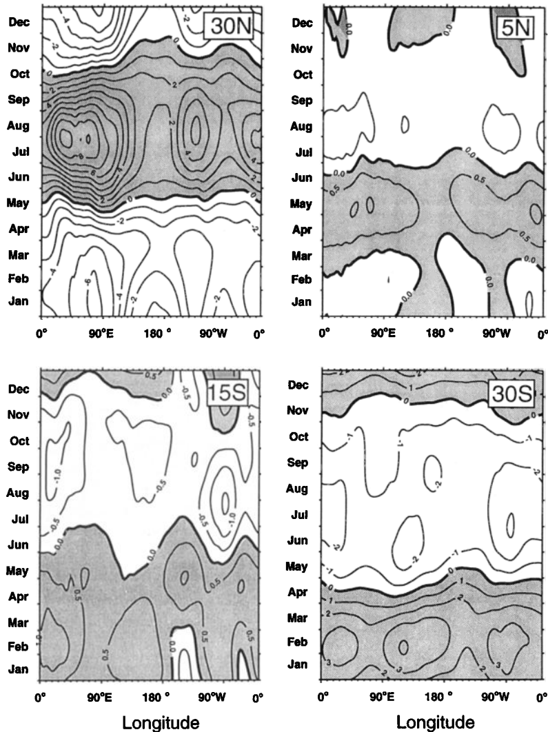
Figure 6b. Longitude-time sections showing the annual cycle of the upper tropospheric (200–500 mbar) temperature anomaly at 30°N, 5°N, 15°S, and 30°S. Plots are extensions of initial calculations first made for 30°N by Li and Yanai [1996]. The anomalies were calculated by subtracting the annual cycle harmonic at a particular latitude from the mean columnar temperature.
