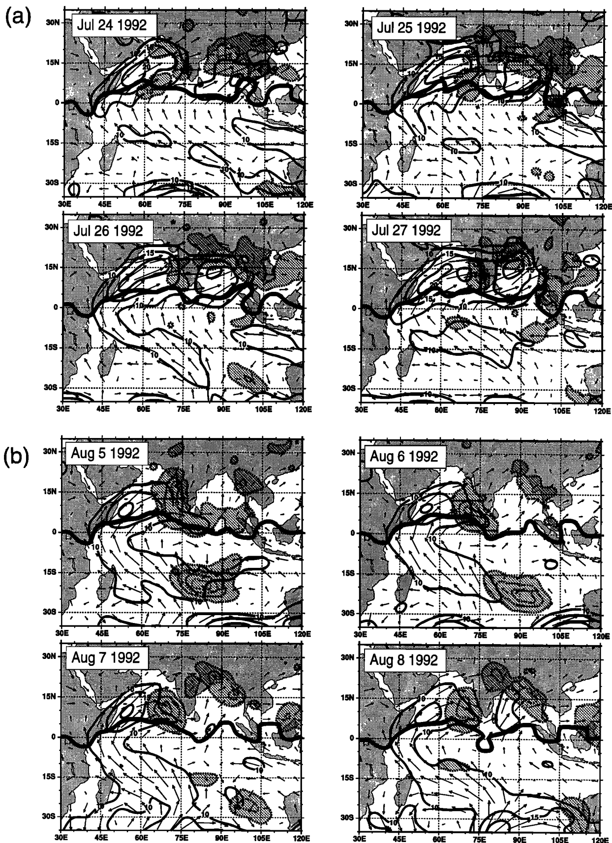
Figure 17. Detailed analyses of 850-mbar velocity (vectors) and precipitation (shaded areas) for two sequences during the summer of 1992 from late July to early August within the dashed rectangles of Figure 15. (a) Four days of an active period (b) four days of a break period. The thick black contour shows the zero absolute vorticity at 850-mbar. See appendix for definition and the timing of the active and break periods. Note the complexity of the individual active and break periods in sharp contrast to the composite reconstructions shown in Figure 16.
