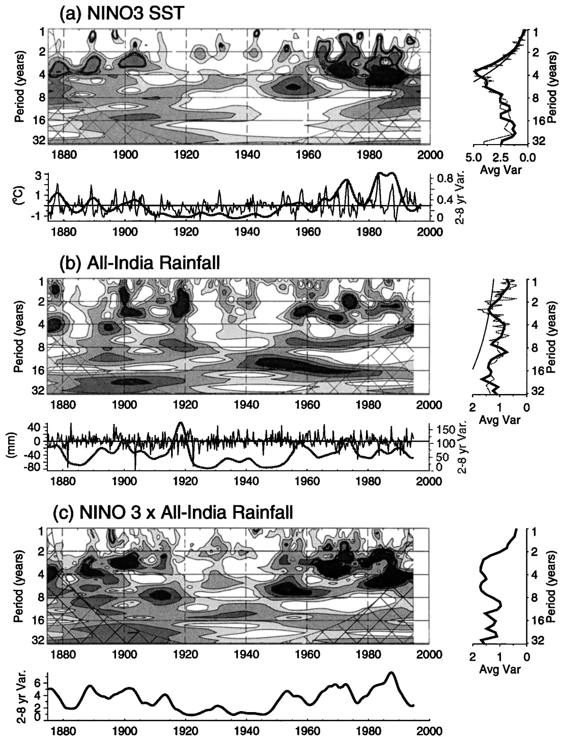
Figure 3. Wavelet modulus analyses of climate time series in the Pacific Ocean and the Indian Ocean. (a) Pacific Ocean sea surface temperature (SST) (1875–1992) in the Niño 3 region (see Figure 14 for location), (b) The all-India rainfall index (AIRI) (1875–1992), and (c) the cross-wavelet modulus between the AIRI and the Niño 3 SST. Contours indicate the percent of total variance at a particular frequency explained at a particular time in the data record. Thick black contours on each modulus indicate that the amplitude within is significant at the 95% level. The dashed areas on the right and left of the moduli distributions indicate the limitations of the data to define variance of a particular period at a particular time of the data record. Below each wavelet modulus is the data record, with a gray curve that represents the percent of the total variance explained at all frequencies at a particular time. The black curve below the cross-wavelet modulus represents the covariance of the AIRI and the Niño 3 SST in the 2–8-year-period band. On the right-hand side of each modulus are periodograms computed in two different ways. The gray curves represent the fast-Fourier Transform of the entire data series. The black curves represent the summed wavelet modulus. The 95% confidence curve is also plotted on the periodograms. Methods described in Torrence and Compo [1998] are used.
