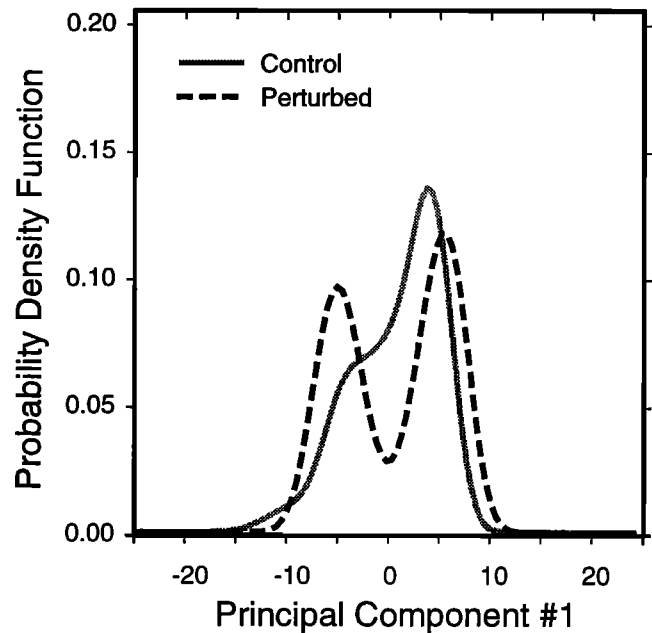
Figure 36. Probability density functions (PDFs) of the vertical velocity structure of the intermediate coupled monsoon model for the control (gray curve) and for a case where a remote climatological forcing was introduced (dashed curve). Different structures result from the external influence. From Dixit et al. [1997] .
