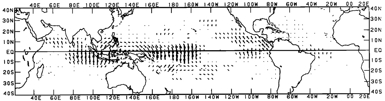
Figure 18. Biennial coherence between the SST in the central Pacific (equator and 170°E) and the zonal wind component over the global oceans represented by harmonic dial vectors. The maximum biennial SST-zonal wind correlation (0.7) is at the base point. The downward (upward) pointing arrows signify in phase (1 year out-of-phase) relationships. From Ropelewski et al. , [1992].
