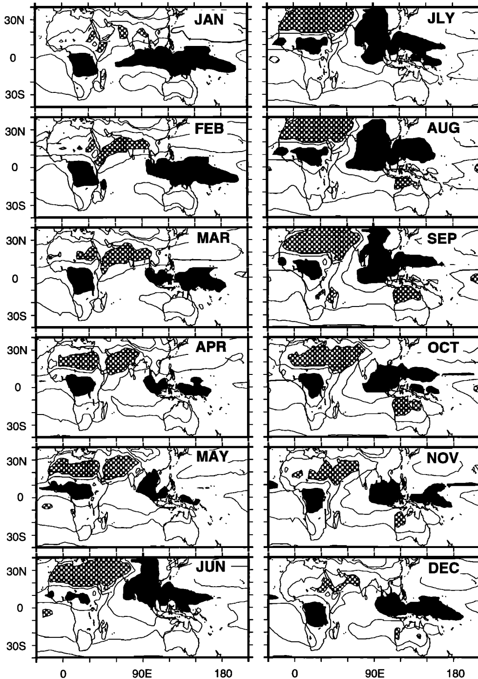
Figure 2. Annual cycle of outgoing longwave radiation (OLR) measured by satellite. Shaded and cross hatched regions indicate OLR < 220 and > 300 \text{ W m}^{-2} , respectively. OLR minima are surrogates for persistent deep convection and latent and radiative heat sources within the troposphere. Regions of maximum OLR, on the other hand, indicate radiative loss to space and hence are heat sinks. An annual migration of the major atmospheric heat sources and sinks of the tropics and subtropics is apparent. After Webster [1995].
