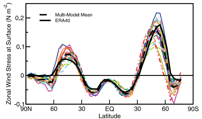
Figure 8.7. Annual mean east-west component of wind stress zonally averaged over the oceans. The observationally constrained estimate is from the years 1980 to 1999 in the European Centre for Medium Range Weather Forecasts 40-year reanalysis (ERA40; Uppala et al., 2005), and the model climatologies are calculated for the same period in the 20th-century simulations in the MMD at PCMDI. The legend identifying individual models appears in Figure 8.4.
