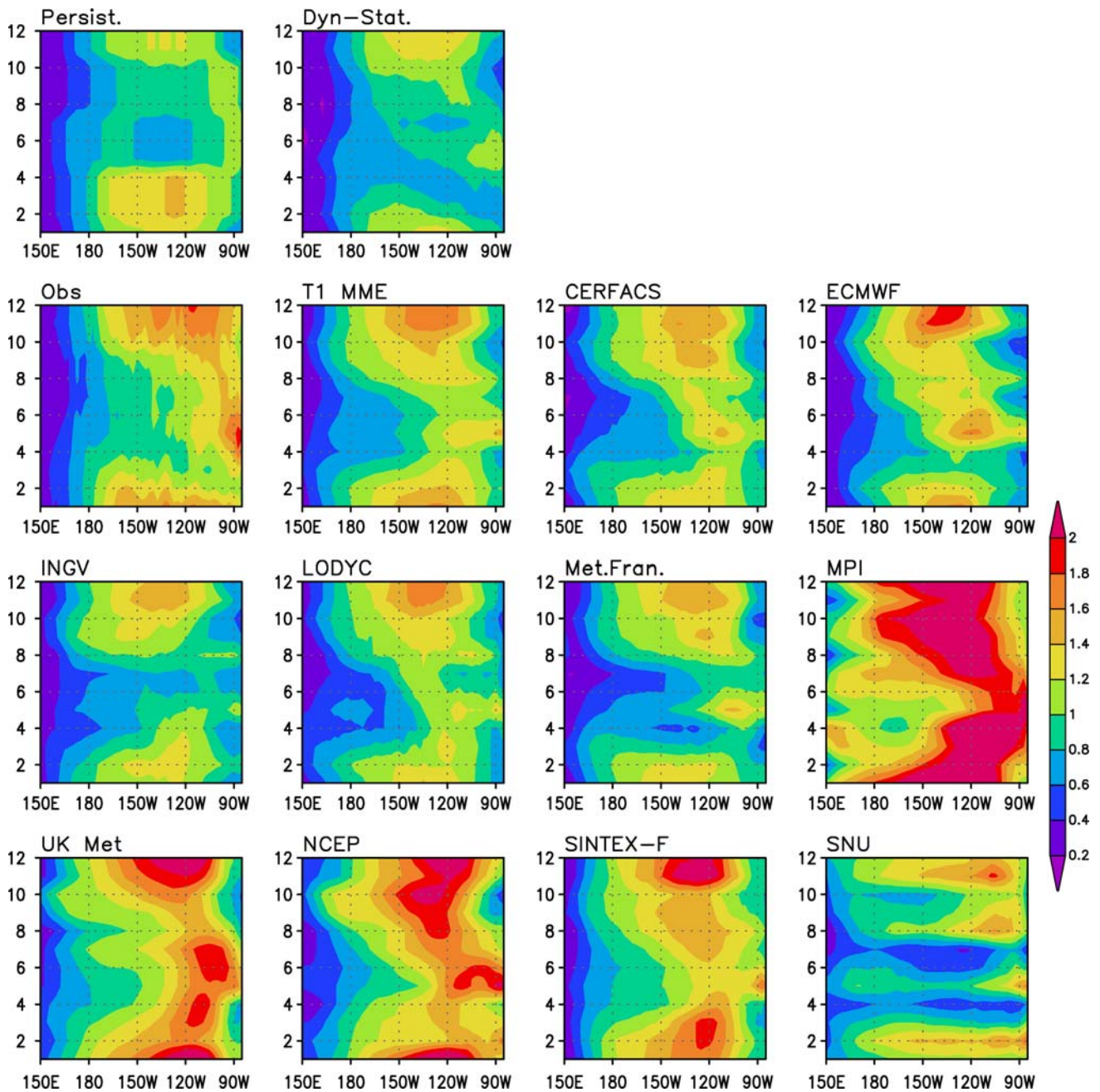
Fig. 4 Observed and simulated standard deviation of SST anomalies as a function of calendar month along the equator (2°S–2°N). For models, the 1- to 3-month-lead forecast data are used
